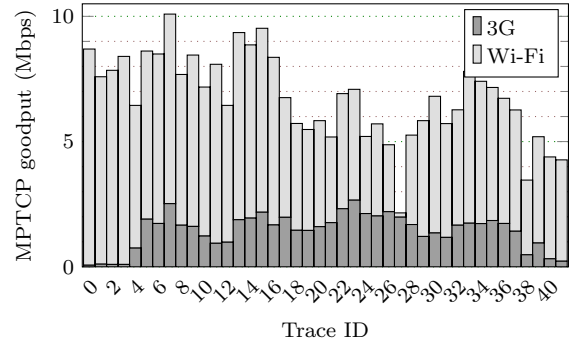
Figure 4: Average MPTCP goodput of all the traces
